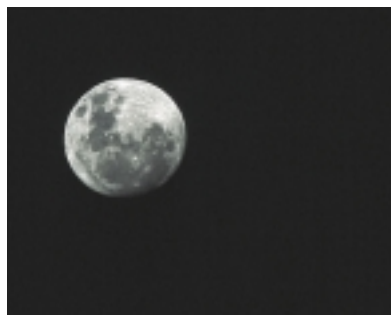
Figure 5.8 Galileo observed the Moon's blemishes, which had shadows that lengthened and shortened with the Sun's angle on them. Galileo concluded that the Moon's surface has mountains and craters on it, much the same as Earth.
