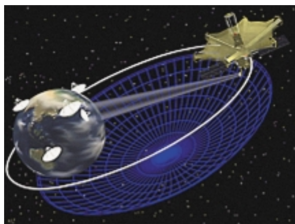
Figure 5.39 Canadian astronomers are participating in an international VLBI project called VSOP (VLBI Space Observatory Program). This project uses a radio dish in space and an array of ground-based telescopes, which simulates a single dish twice Earth's diameter! Astronomers at the University of Calgary calibrate and image some of the data for this program. This telescope has been able to image objects over 13 billion light-years from Earth.
