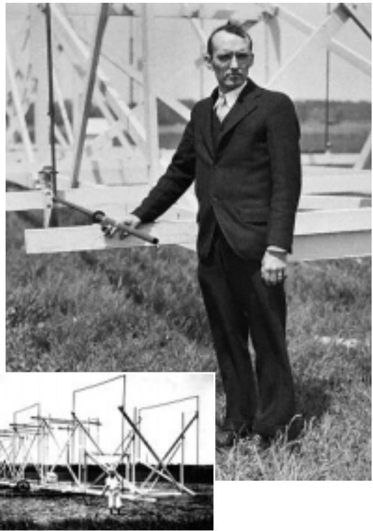
Figure 5.34 The world's first radio telescope (inset) by Karl Jansky, marked a big moment in science as was Galileo's optical telescope 300 years before.
